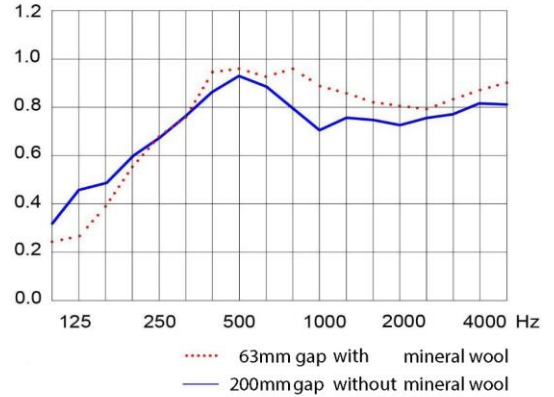
Absorption according to EN ISO 354
